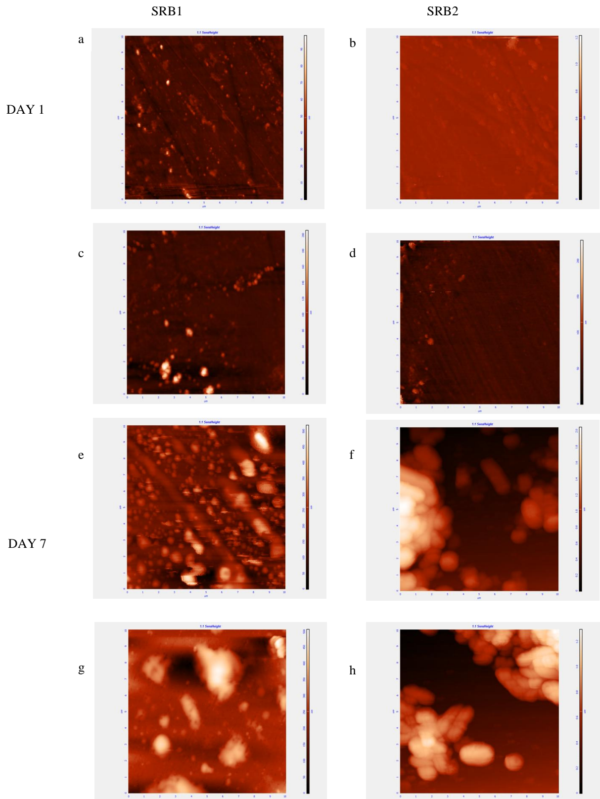
Figure 2a: AFM image of biofilm formation on AISI 304 stainless steel for SRB1 (a, c, e & g) & SRB2 (b, d, f & h) for day 1 ; (a), (b), (c) & (d) day 7 ; (e), (f), (g) & (h). Magnification 10 \mu\text{m} x 10 \mu\text{m} .
