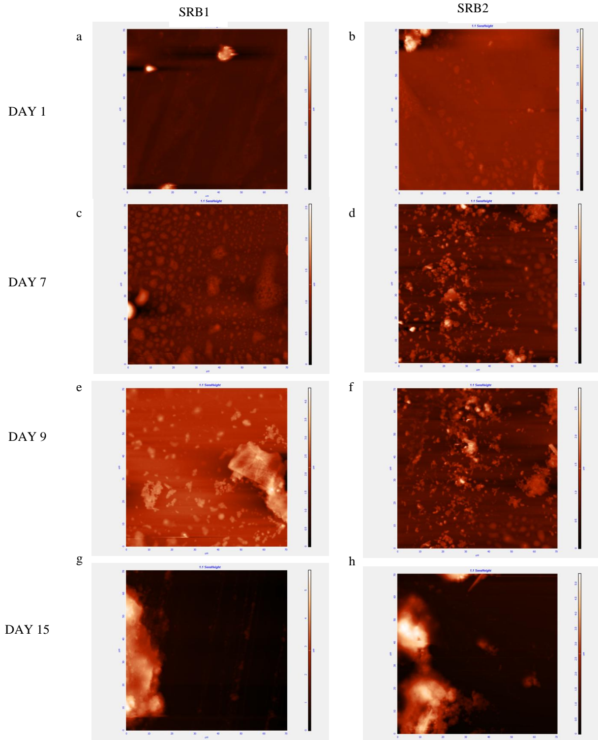
Figure 1: AFM image of biofilm formation on AISI 304 stainless steel for SRB1 (a, c, e & g) & SRB2 (b, d, f & h) for day 1 ; (a) & (b), day 7 ; (c) & (d), day 9 ; (e) & (f) and day 15 (g) & (h). Magnification 70 \mu\text{m} x 70 \mu\text{m} .
